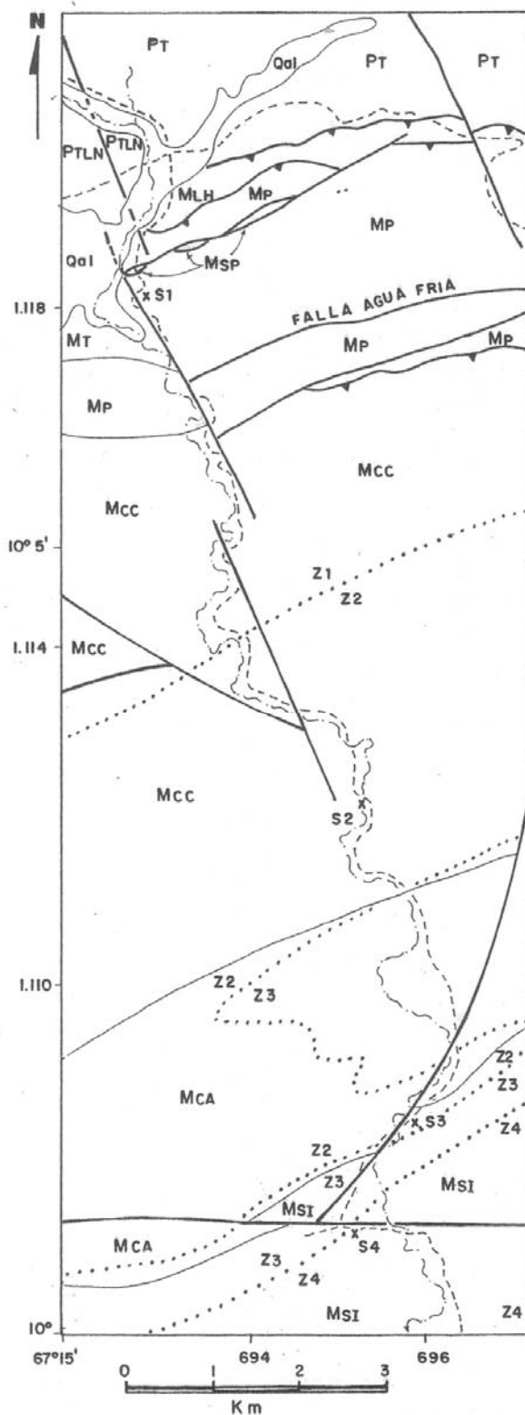
Fig. 15. Geological map of the Río El Pao section, between El Pao de Zarate and San Sebastián.
