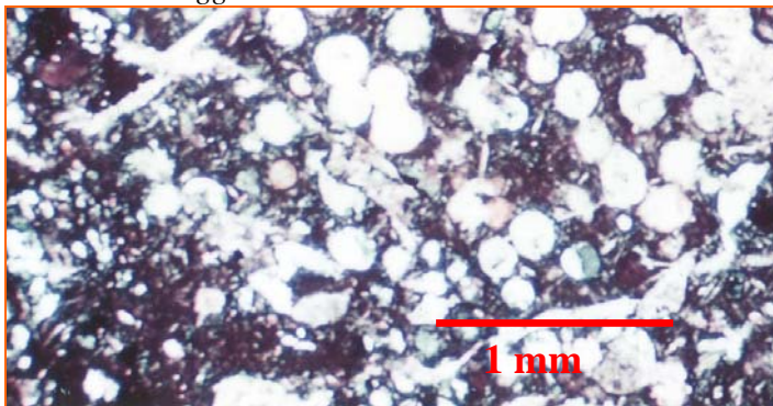
Fig. 20d. Amigdaloid lava. Right from a thin section: vesicles filled by quartz chlorite calcite and pumpellyite (LUGO 1982:140)
