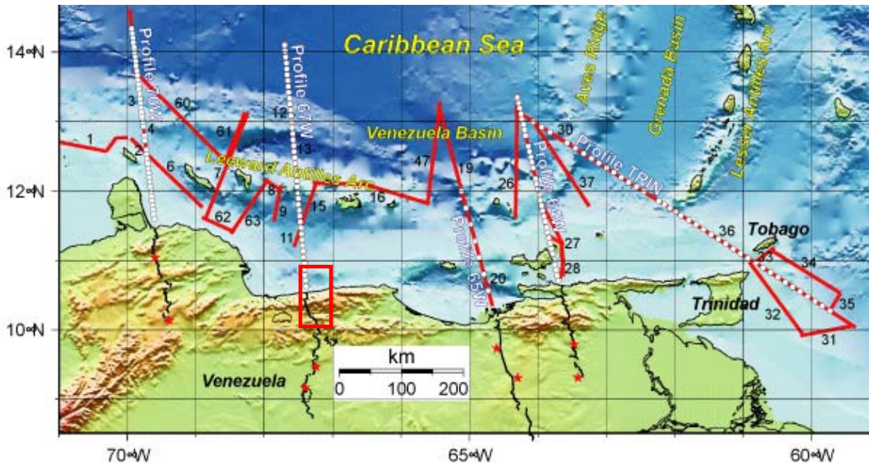
Fig. 1. BOLIVAR and GEODINOS transects. The red rectangle shows the area to be visited.
