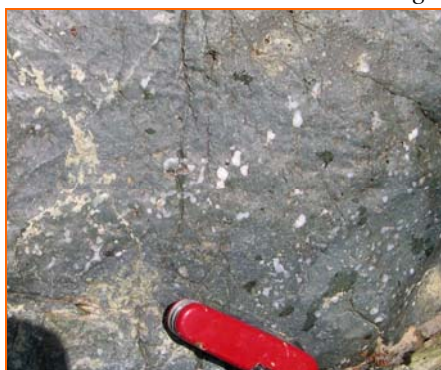
Fig. 20d. Amigdaloid lava. Right from a thin section: vesicles filled by quartz chlorite calcite and pumpellyite (LUGO 1982:140)
