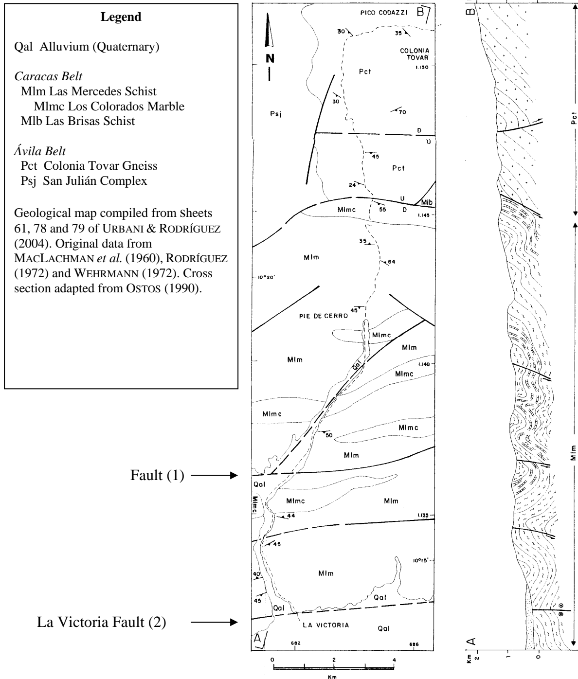
Geological map and cross-section of La Victoria - Colonia Tovar, Aragua state.
