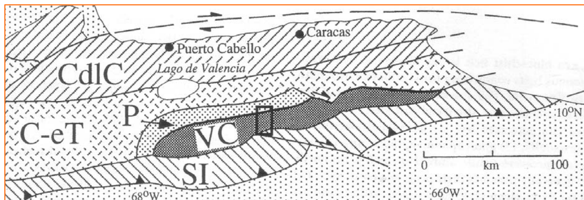
CdlC - Cordillera de la Costa, C-eT - Caucagua El Tinaco belt, P - Paracotos belt, VC - Villa de Cura belt, SI - Serranía del Interior foreland and thrust belt.
