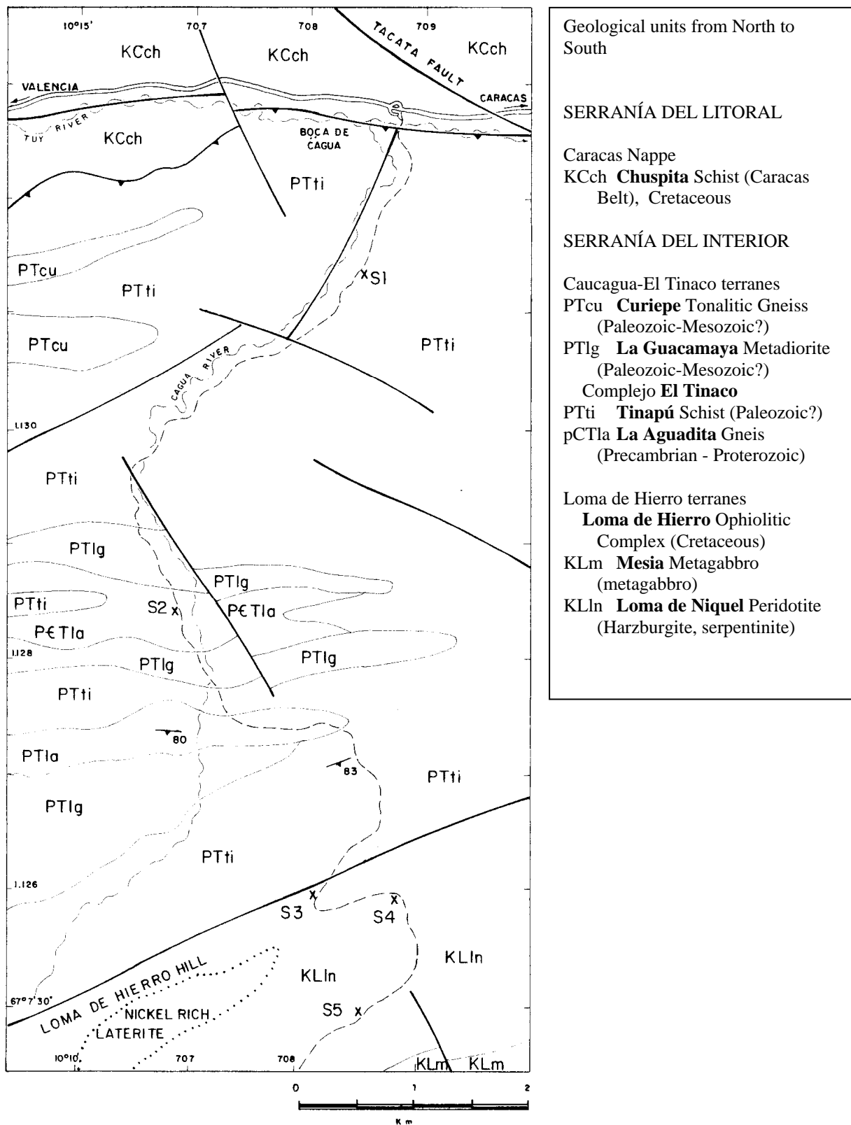
Fig. 8. Geological map of Boca de Cagua – Tiara section. Simplified from sheet 67 and 70 of URBANI & RODRÍGUEZ (2004), with original data from SMITH (1953) and BECK (1985).
