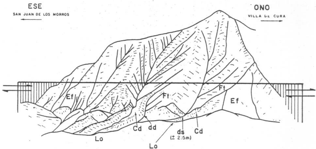
Fig. 2. Geomorphic evidence of recent tectonic activity along the Río Guárico fault (From AUDEMARD et al. 1989).
